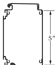
2 Piece 5" Narrow Channel Letter Raceway
