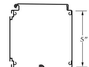
2 Piece 5" Channel Letter Raceway
