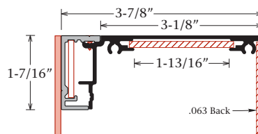
Series 4 Single Face Access Body Part #1391 Frameless Cover Part #1693
