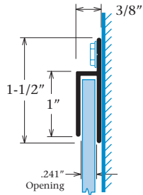
1" H-Molding Part #1945
