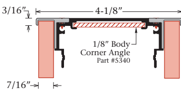
Extended Insert End Cover Part #1698
