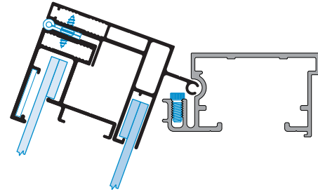
2Part Large Outer Frame Part #1941
