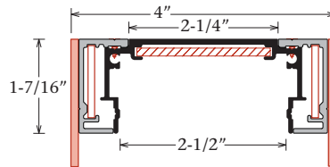
Series 4 Access Body Part #1390 Frameless Cover Part #1693
