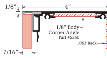
Insert End Cover Part #1696
