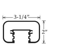
Rectangular Post w/Radius Edges *Part #1230
