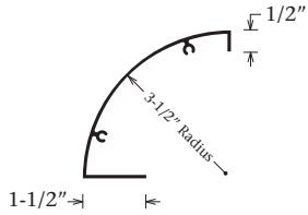
3-1/2" 1/4 Round End Part #1670
