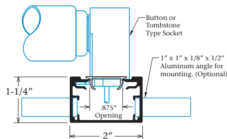
Socket Raceway Part #1984 Socket Raceway Cover Part #1987
