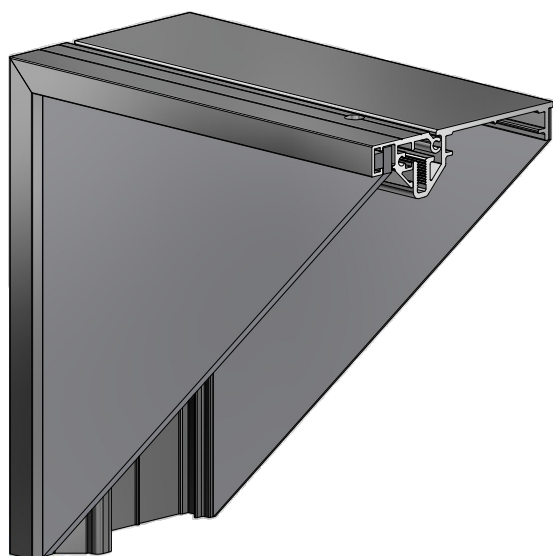
Series 4 SF Hinge Body w/ 1/2" Slide Retainer
