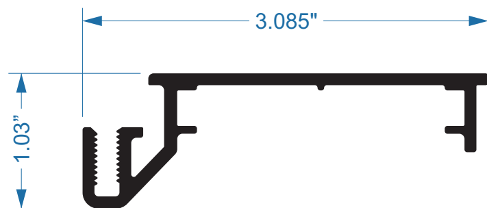
SERIES 4 SINGLE FACE HINGE BODY #1601 SCALE: FULL SIZE
