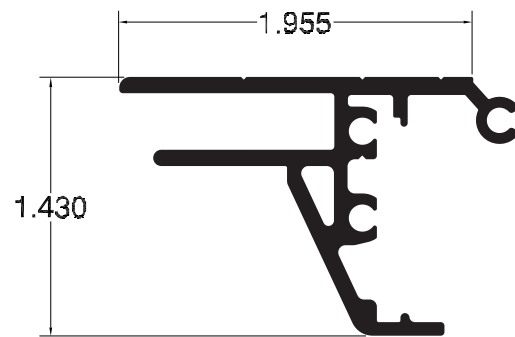
Frameless Rigid Retainer Part# 1628
