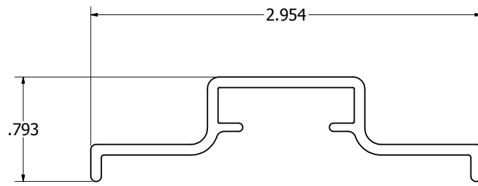
5" NARROW CHANNEL LETTER RACEWAY LIFTING BRACKET PART# 1975N
