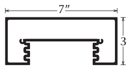
Rectangular Post Part #1510
