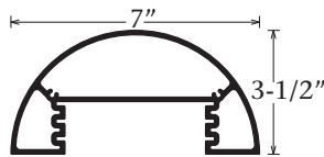
Radius Post Part #1500
