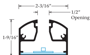
Edge Lit LED 1/4 Round Part #1996
