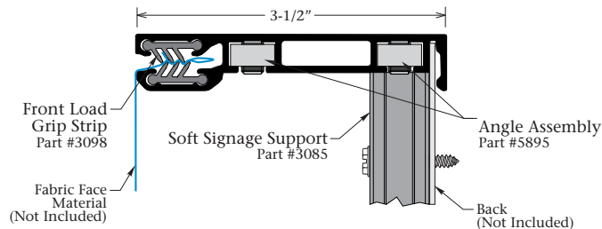
3-1/2" Front Load Soft Signage Frame Part #3095A
