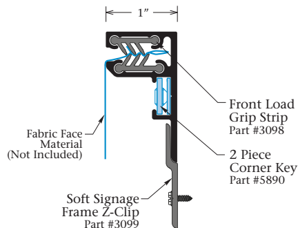
1" Front Load Soft Signage Frame Part #3092A
