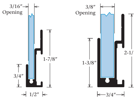
3/4" Wall Frame Part #1948
