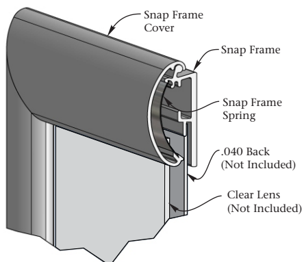
Snap Frame Part #1899 Snap Frame Radius Cover Part #1896A Material Thickness Range: .000 - .125
