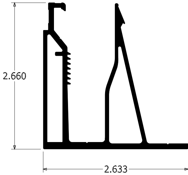
Front Load Wall Mount Tension Frame #2080
