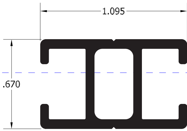
Soft Signage Support Part #3085
