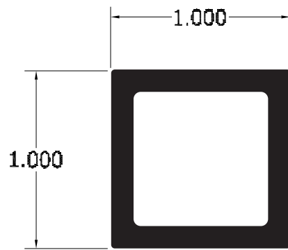
Small Frame Support Tube 1" Part# 2177
