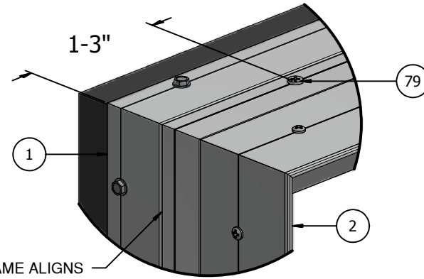
DETAIL A FRAME CLOSED
