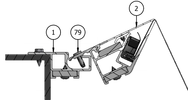
TOP CROSS-SECTION VIEW
