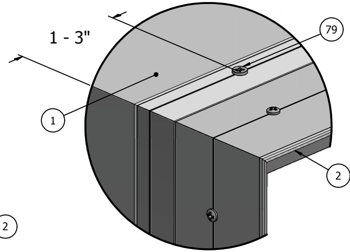
DETAIL A FRAME CLOSED
