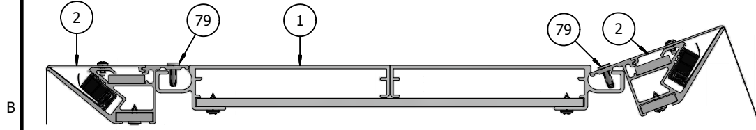
TOP CROSS-SECTION VIEW
