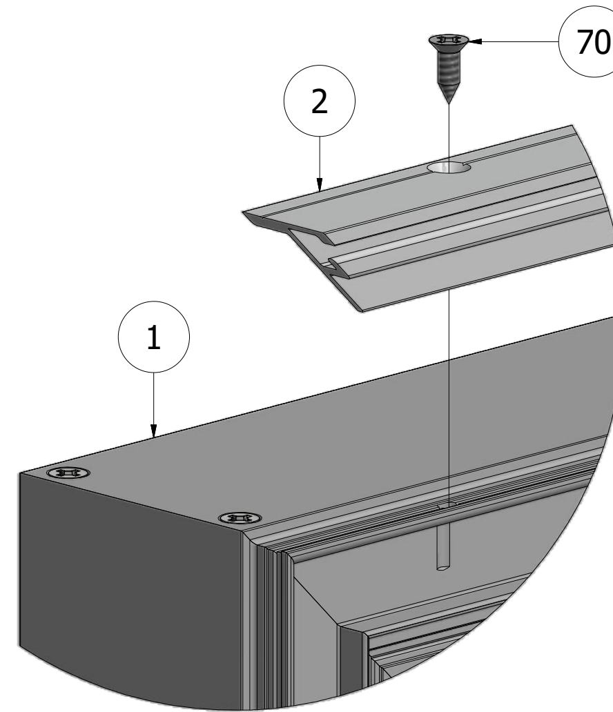
DETAIL A-1
