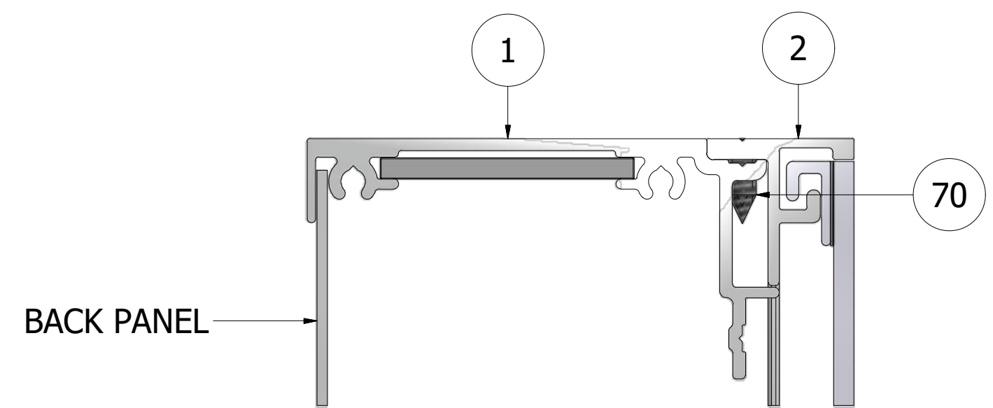
TOP CROSS-SECTION
