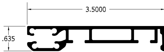
3-1/2" Front Load Soft Signage Frame Part #3095
