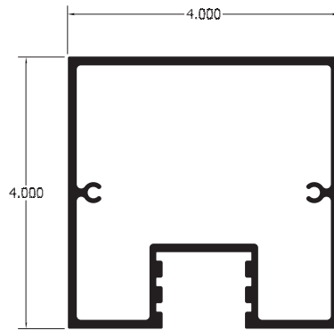
SERIES 4 4IN SQUARE POST #1333
