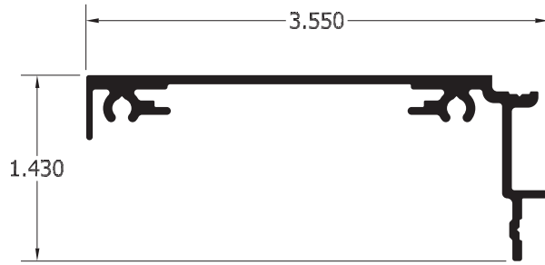
SERIES 4 SINGLE FACE ACCESS BODY #1391
