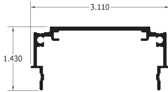
SERIES 4 ACCESS BODY #1390
