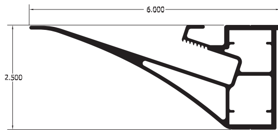
6" Flat Bleed Single Face Tension Body Part #2233
