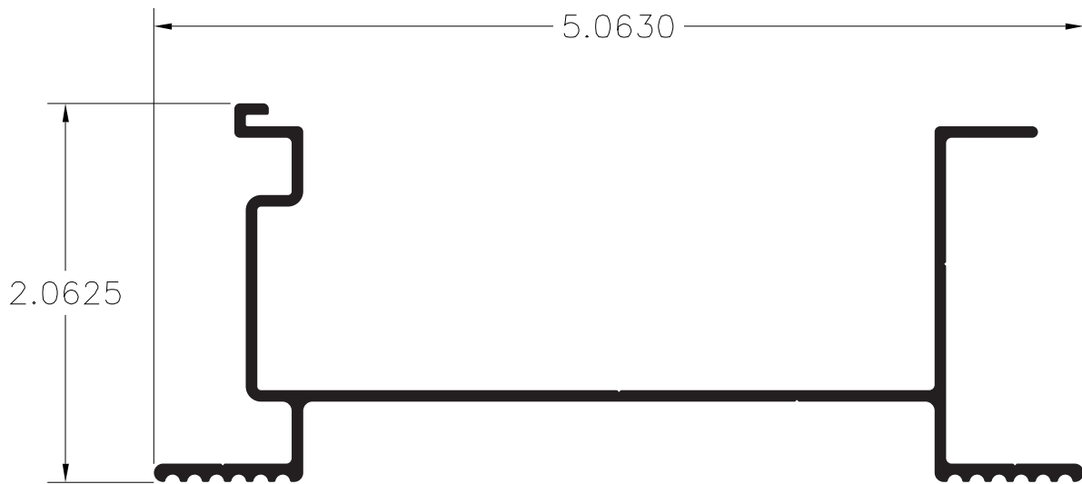
Ballast/Power Supply Raceway Part #1969
