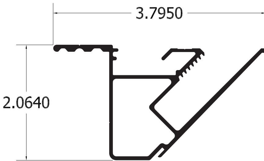
Flat Bleed Retro Frame w/ Reflector Slot Part #2103
