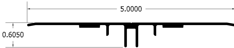
Flat Bleed Double Face Tension Cover Part# 2235
