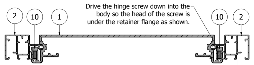
TOP CROSS-SECTION
