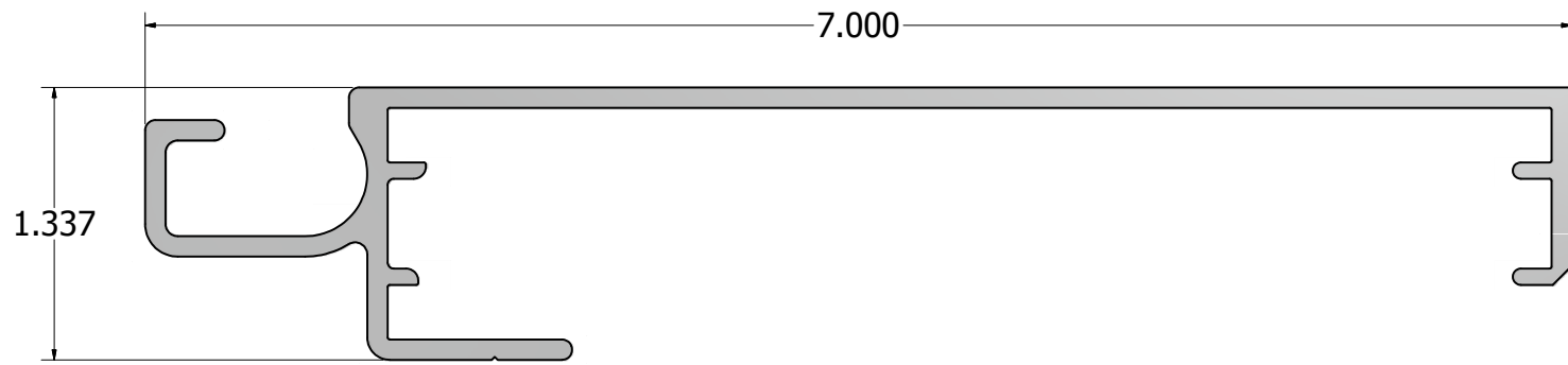
FLAT 2 PIECE NARROW DOUBLE FACE BODY PART# 2010
