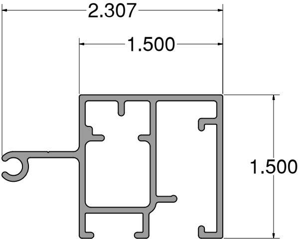
1-1/2" Retainer Part# 2053
