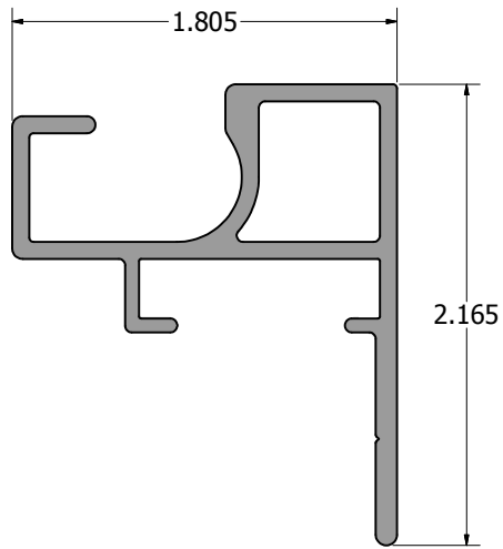
Wall Mount Retro Body Part# 2042
