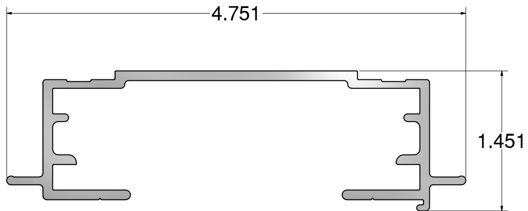
2Part 6" Double Face Body Part# 1936
