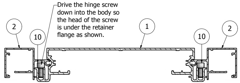
TOP CROSS-SECTION
