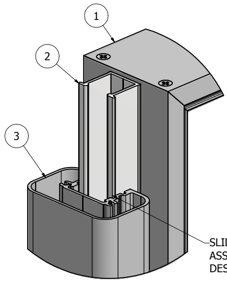
DETAIL A
