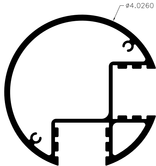
Series 4 90 Deg, Round Post Part #1339
