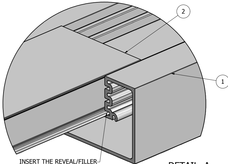
DETAIL A
