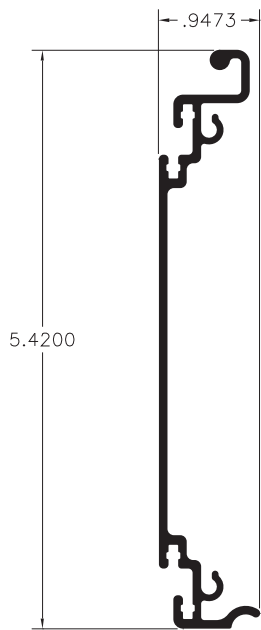
5" Narrow Channel Letter Raceway Back Part #1972N
