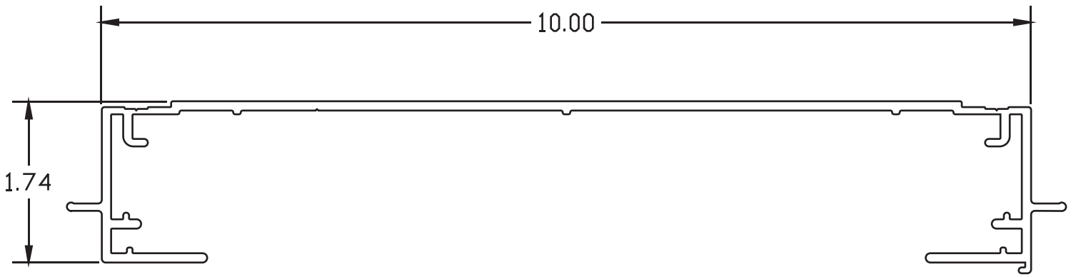
2 PART 12" BODY #1929 SCALE : 1" = 1"
