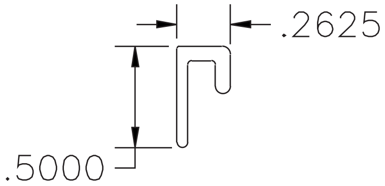
Plastic Insert Panel Adaptor #1689
