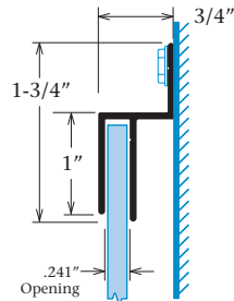
1" Z-Molding Part #1946
