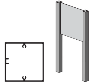
3-1/4" Square Post Part #1005 K1005
