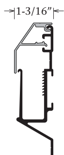
Wall Mount Tension Frame Beveled Cover Part #2091 K2090/91
