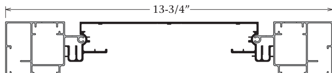
One Side Removable w/ Dual Frame, Part #2065 2-1/4" Dual Frame Cover, Part #2075
