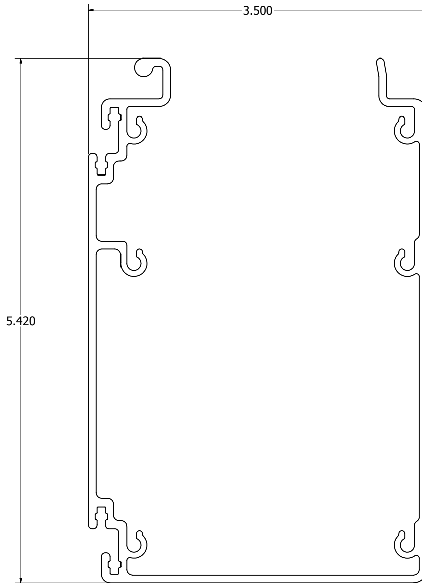
1 PIECE 5" NARROW CHANNEL LETTER RACEWAY PART# 1970N
