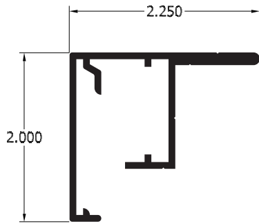
Flat 2" Retainer Part #2047
