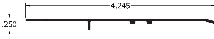
Extended Flat Bleed Retro Frame Cover II Part #2124
