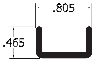
CHANNEL LETTER RACEWAY U-CHANNEL PART#1978
