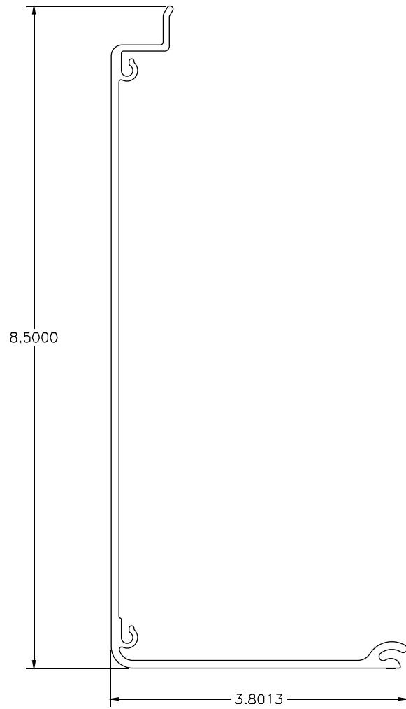
8" 2 PIECE CHANNEL LETTER RACEWAY PART (FRONT) # 1981
