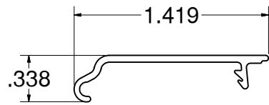
Soft Signage Snap Tension Frame Cover Part# 3094
