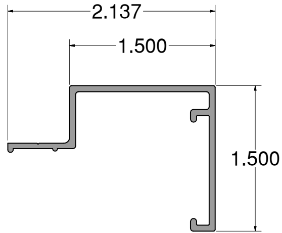
1-1/2" Frame Cover Part# 2073
