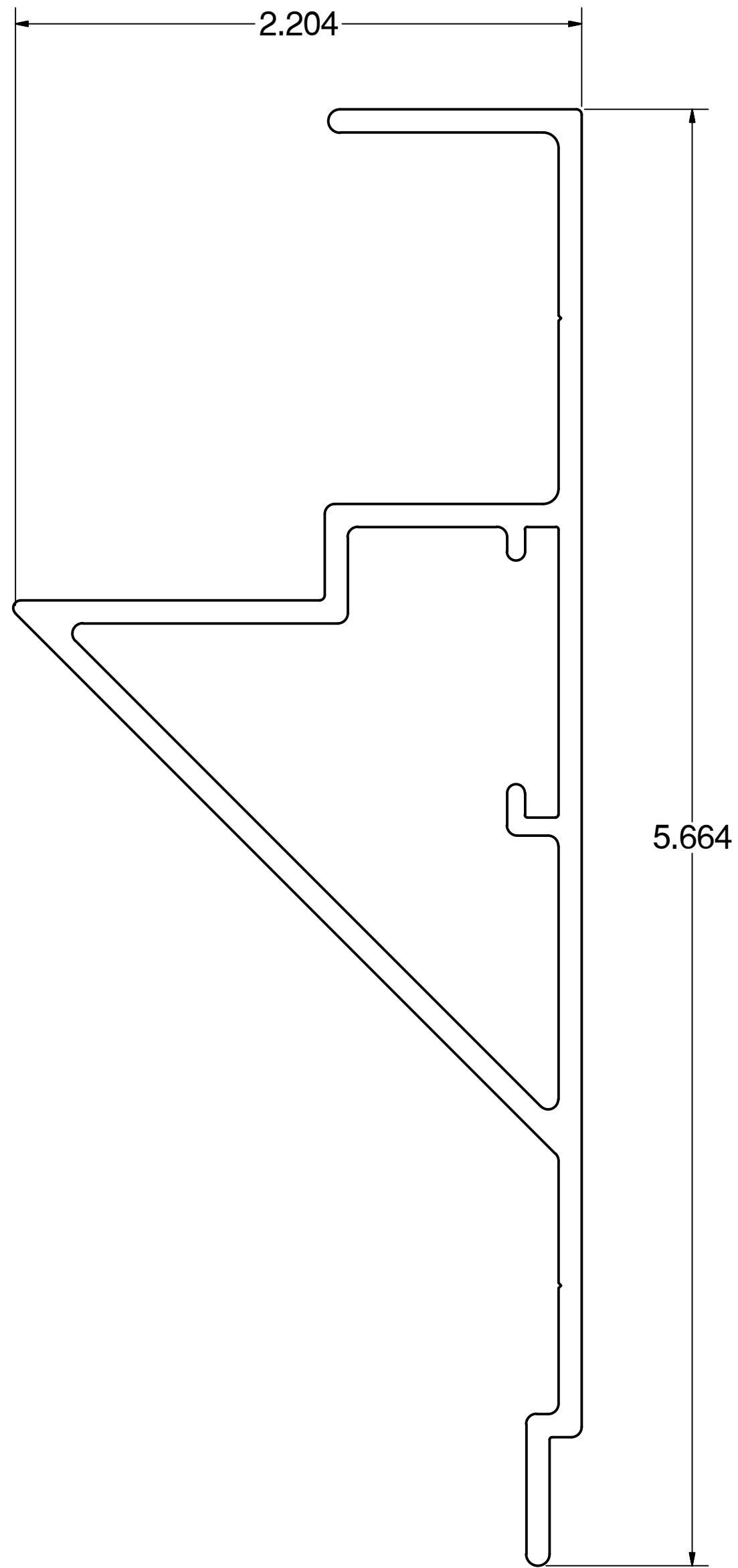
Wall Mount Frame #2100 SCALE 1:1
