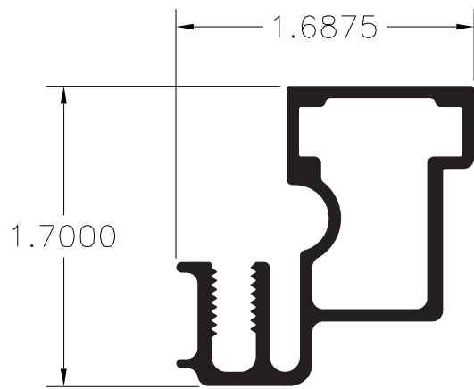
Slimline Single Face Body Part #2020
