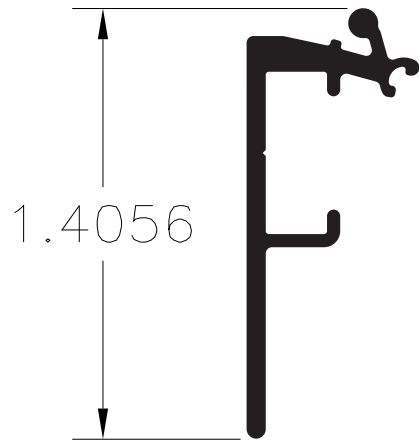
Lg Snap Frame Part #1898
