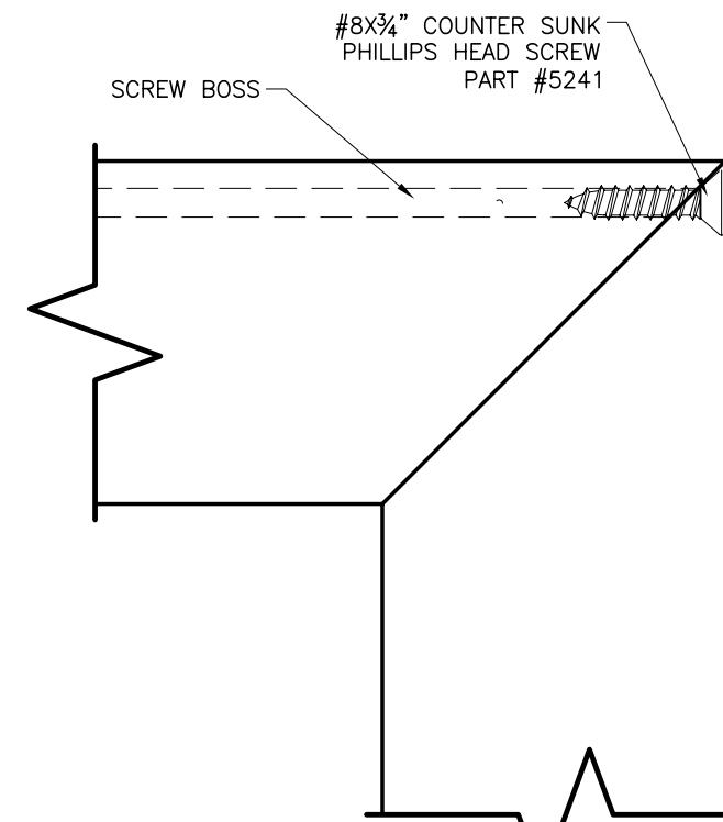
B FACE VIEW SCALE : 1"=1"
