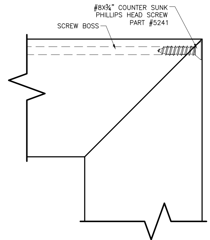
B FACE VIEW SCALE : 1"=1"
