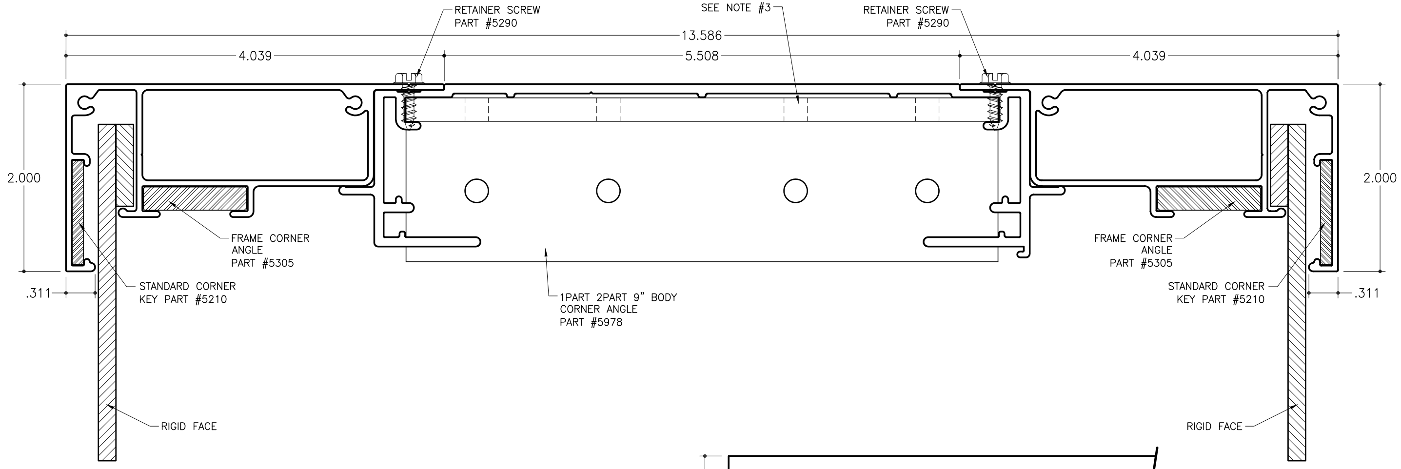
CORNER SECTION DETAIL (ADHESIVE BONDED)
