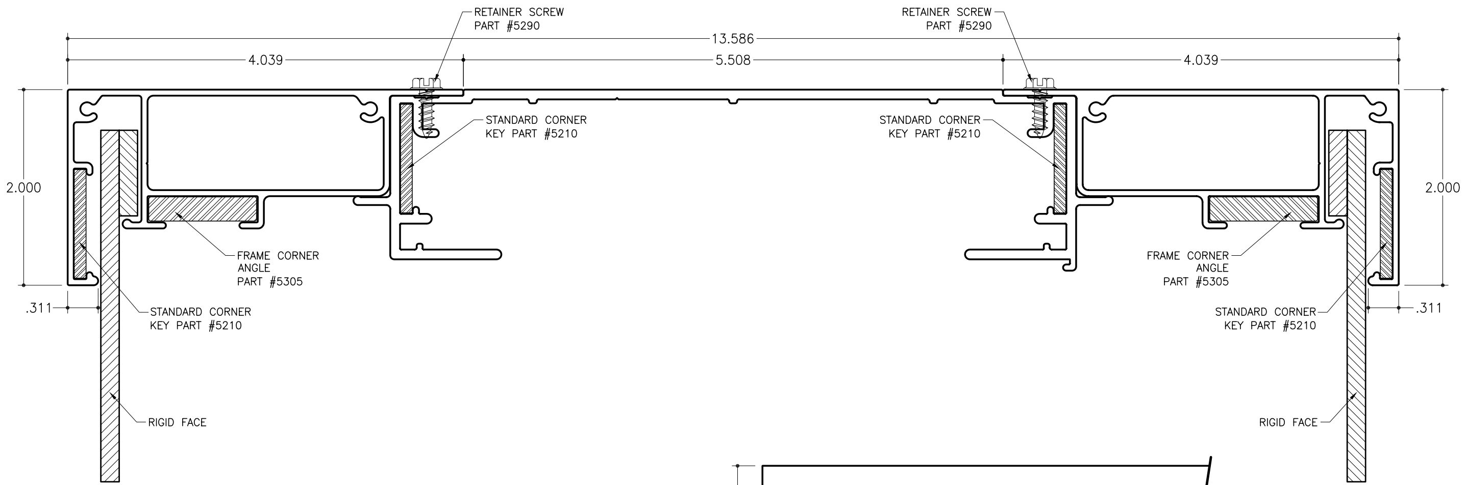
CORNER SECTION DETAIL (WELDED/CORNER KEYS)
