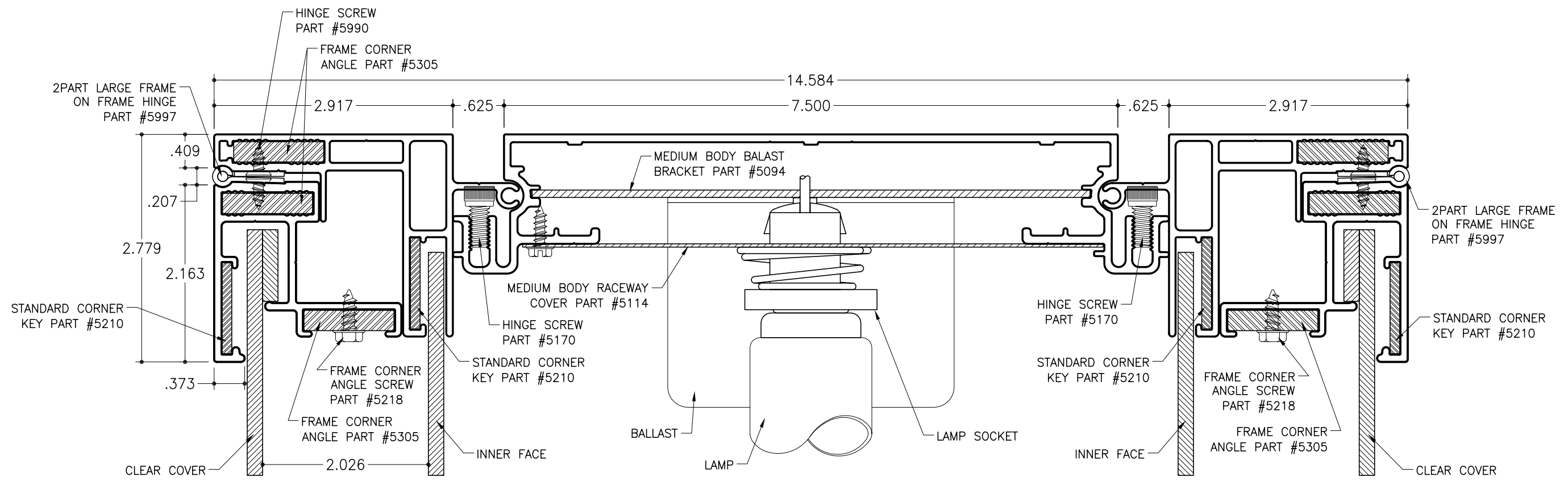
SECTION DEATIL (ELECTRICAL) SCALE : 3/4"=1"
