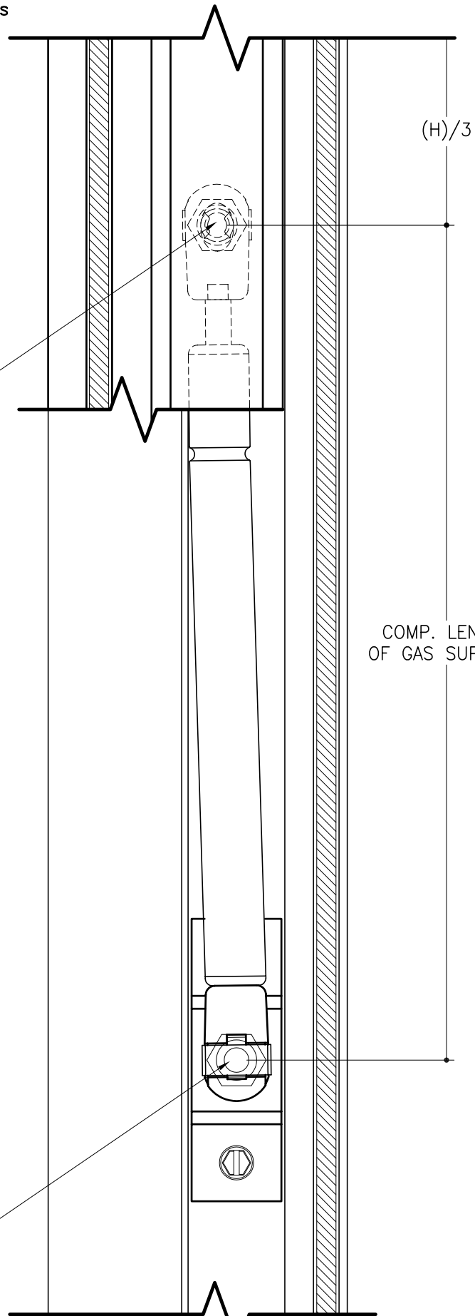
A SECTION VIEW (INSIDE SIDE) SCALE : 3/4" = 1"
