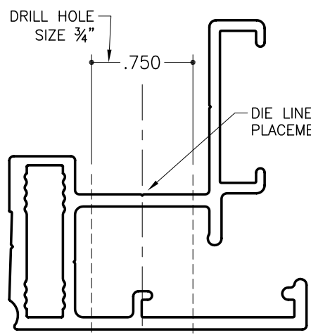
LOCK HOLE DETAIL
