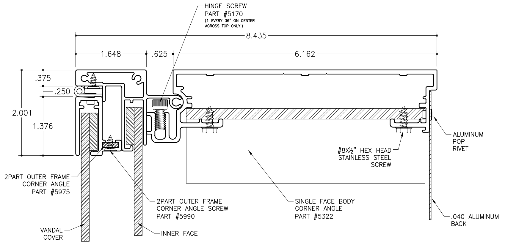
SECTION DETAIL SCALE : 3/4" = 1"
