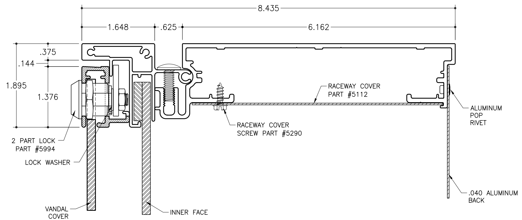
A SIDE SECTION DETAIL SCALE : 3/4"=1"
