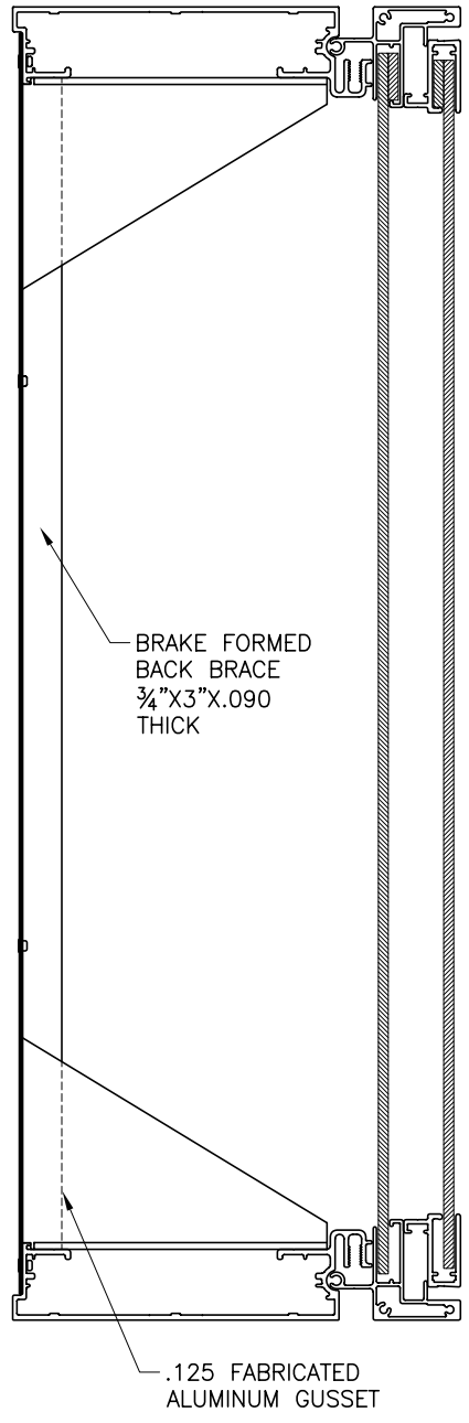
FULL SECTION SCALE : 3" = 1"
